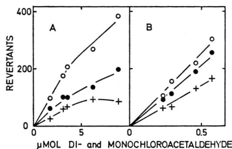
Fig. 1. Reversion of TA 100 with (A) dichloroacetaldehyde and (B) chloroacetaldehyde. ○, without S-9 mix; ●, with S-9 mix lacking NADP and glucose-6-phosphate; +, with complete S-9 mix (20 μl S-9 per plate).
